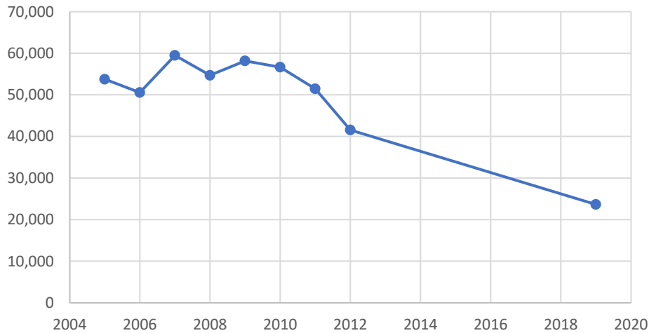
Fire Station Natural Gas Usage (Therms)
